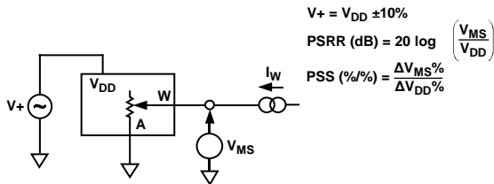
Figure 23. Power Supply Sensitivity (PSS, PSRR)
